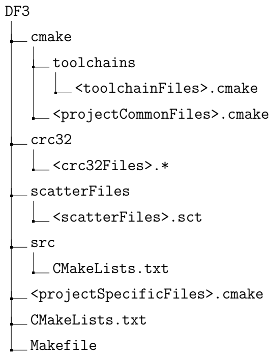
Figure 3.1: General Project Directory Structure
